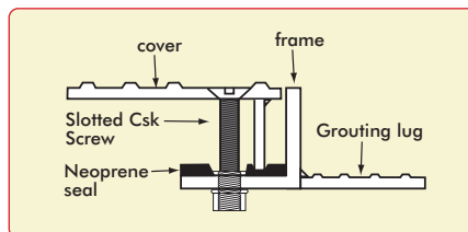
DOUBLE SEAL
